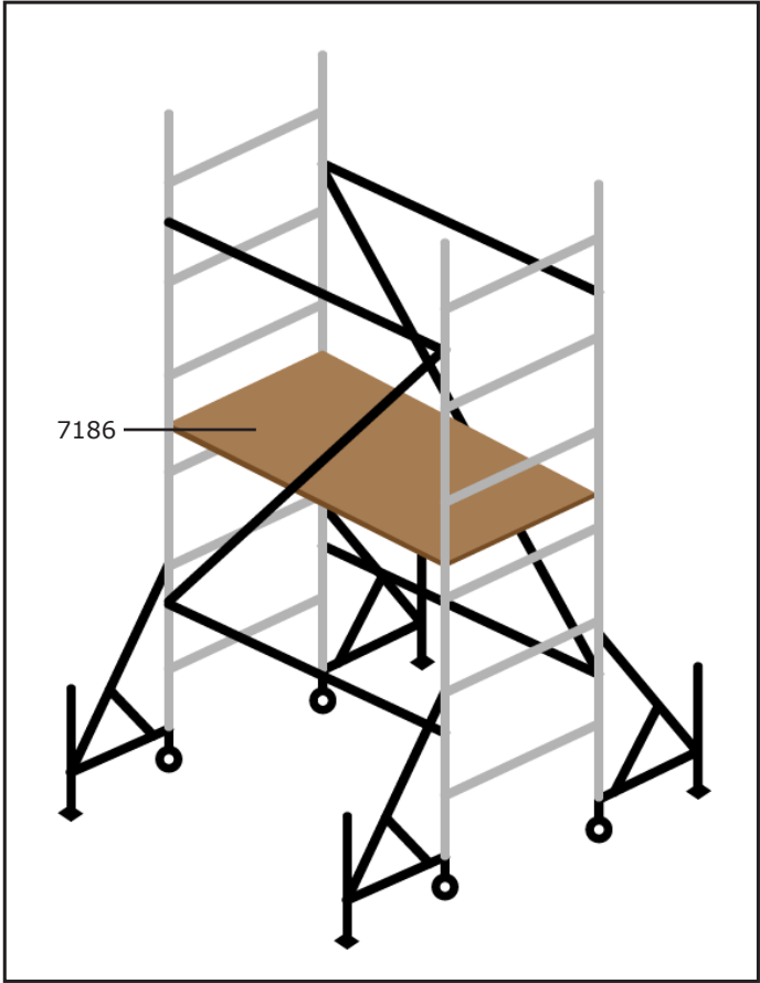
FIG 2. Assembly Diagram (first level)
