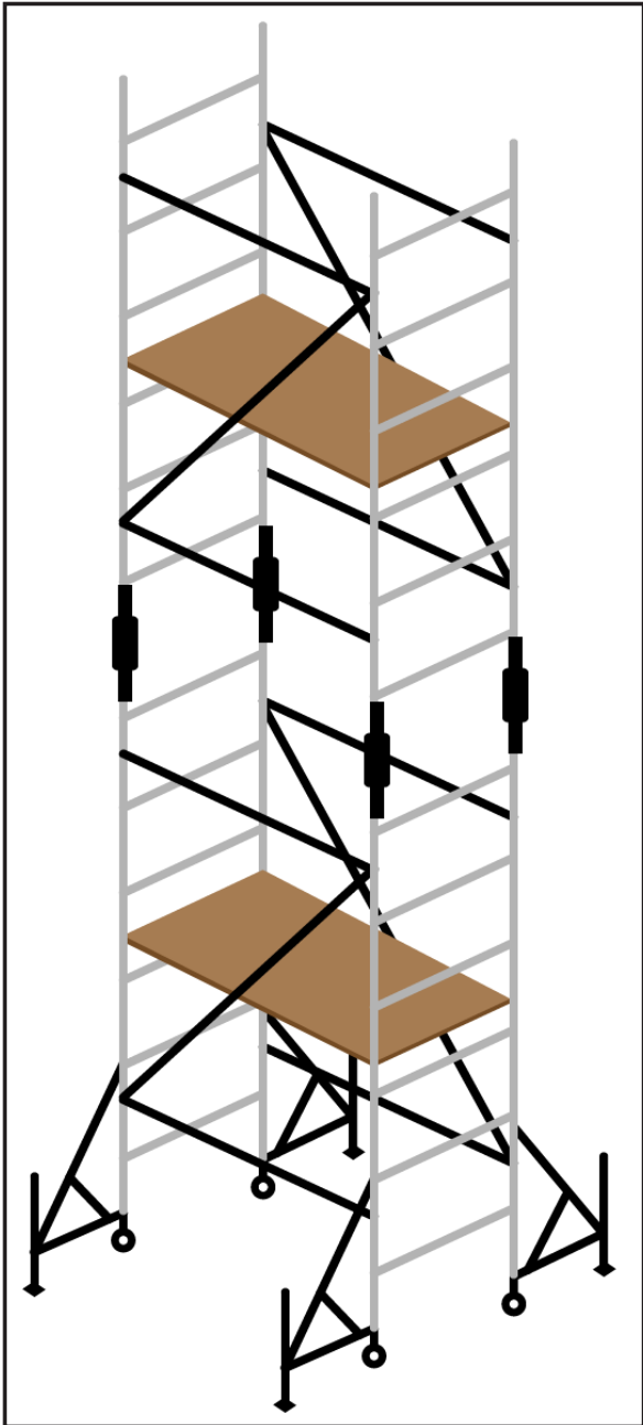
FIG 3-5. Assembling the next structure level with the Scaffold Connectors – M [7171] between the Scaffold Ladders – M [7170]. Repeat process to create a three-tier structure.
