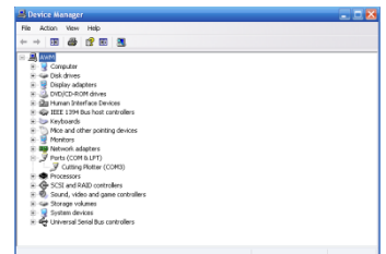
Figure 29: Device manager
