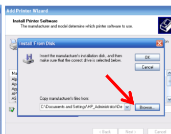
Figure 52: Browse option
