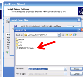
Figure 53: Locate file
