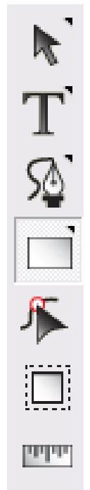
Figure 37: Tools
