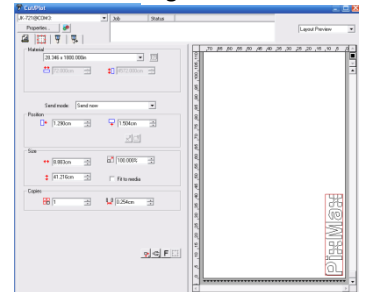
Figure 44: Contour map
