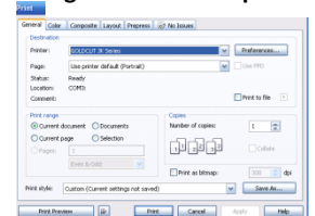
Figure 63: Select printer
