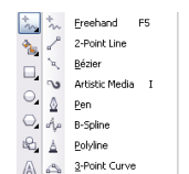
Figure 60: Bezier tool
